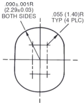
A positive mechanical detent is built into the cam rod shown here in cross section.
