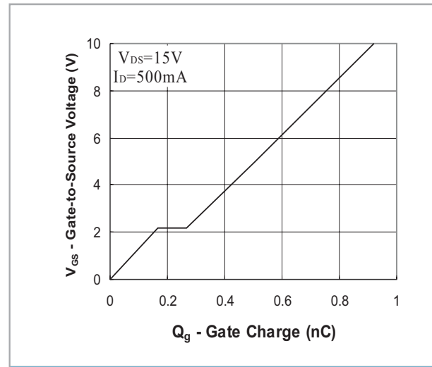
Fig.7 - Gate Charge
