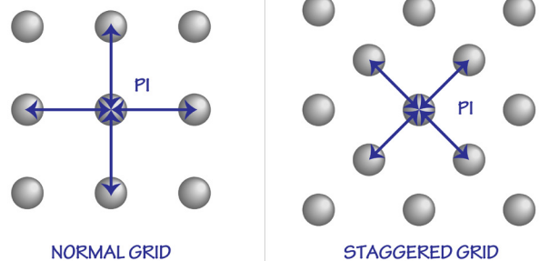
Figure 3 Array (Ball) Pitch
