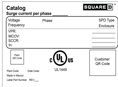
Figure 1 – EMB Nameplate
