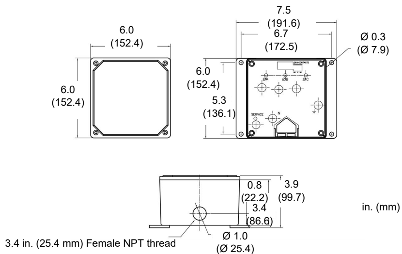
Figure 11: General Dimensions
