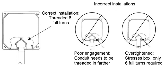
Figure 4 – Conduit Installation
