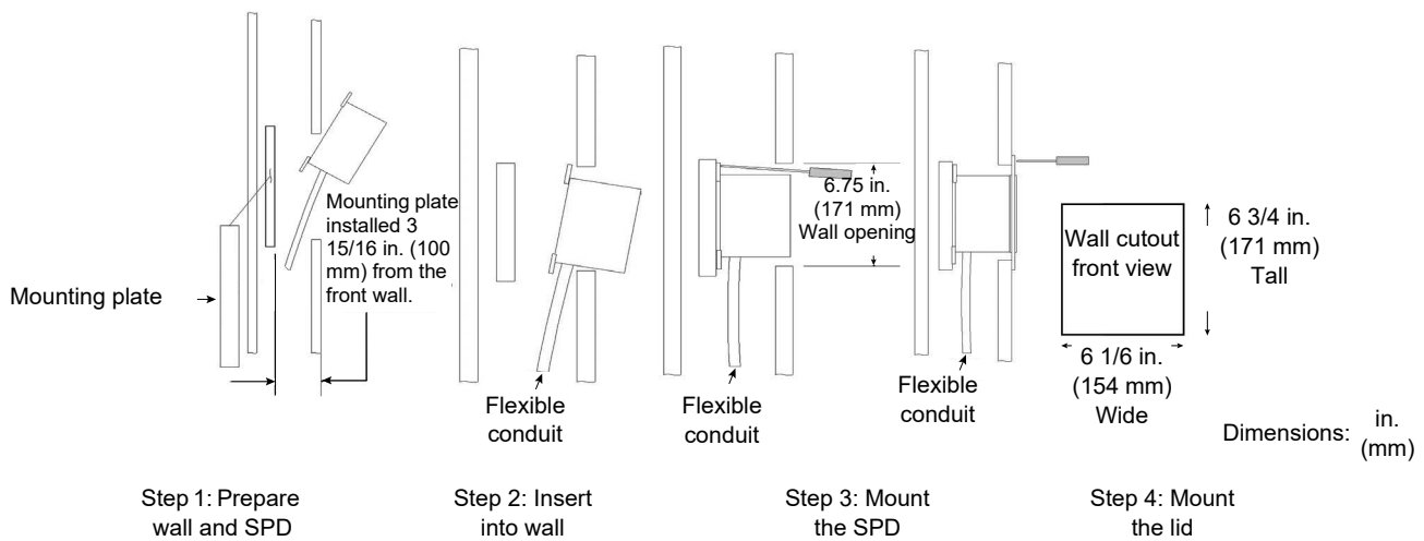
Figure 12 – Flush Mount
