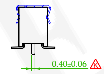
Inner Peg
