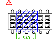
Special CAP for 2*4P 2*5P 2*6P With Bump
