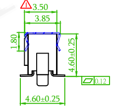
Outer Peg
