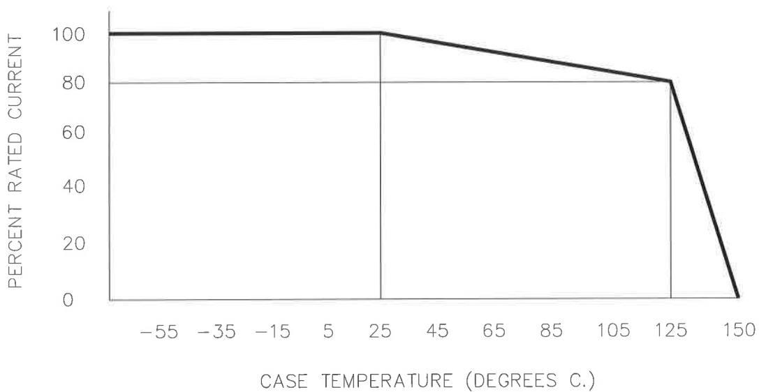
FIGURE 3. CURRENT DERATING LIMITS.
