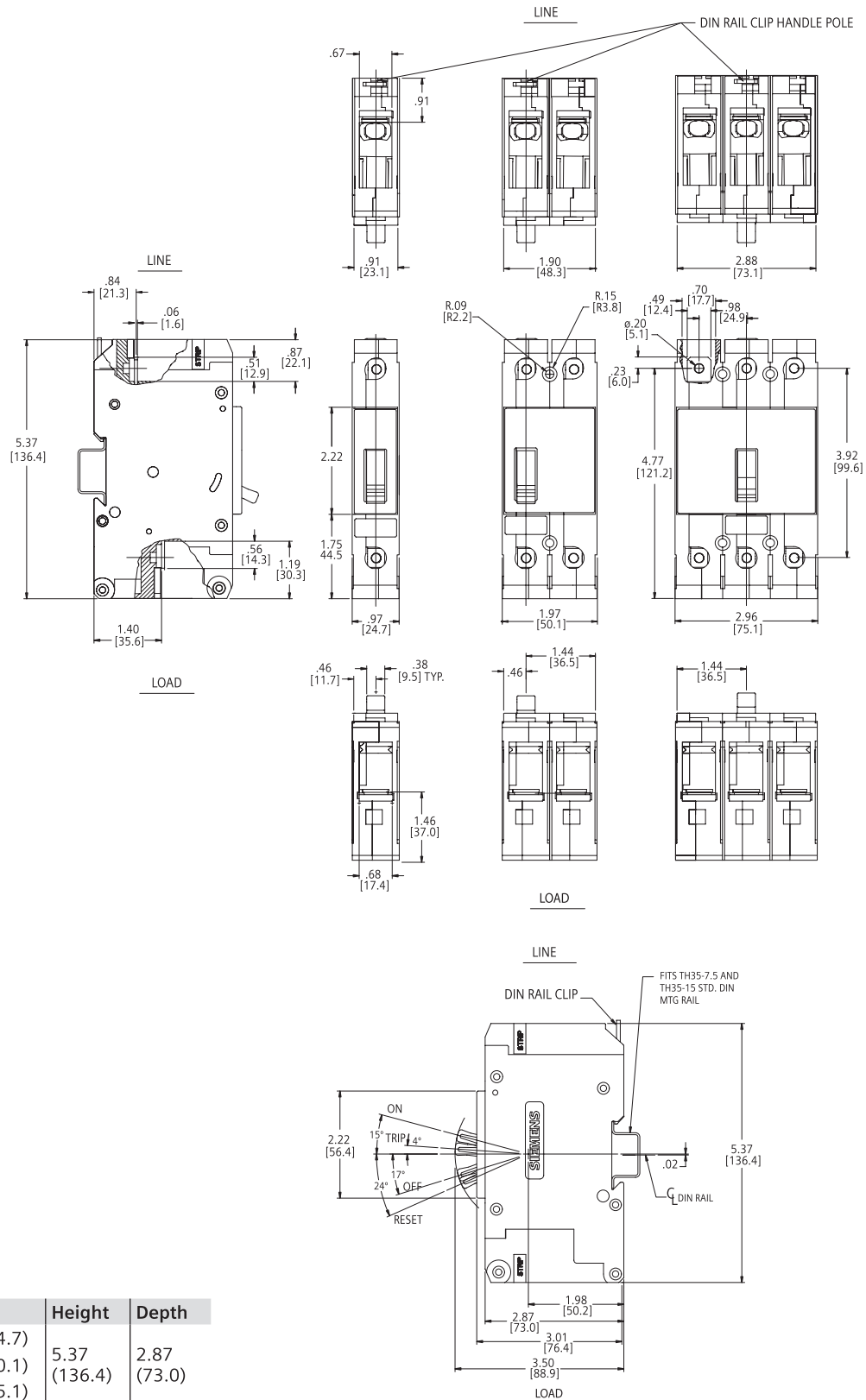
GG Frame Outline Drawing – 1, 2, 3 Pole
