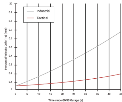
► Horizontal Velocity Drift after loss of GNSS (post INS alignment)
