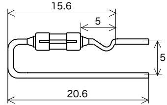
Forming No. F006
