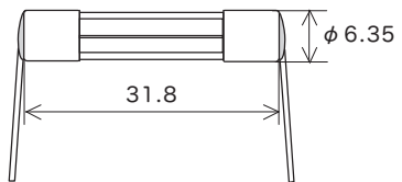
Lead wire diameter φ 0.8 (100 mA–8 A) φ 1.0 (Over 8 A–15 A) φ 1.2 (Over 15 A–20 A) Scale: 1/1 (mm)
