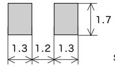
Land pattern for reflow soldering (reference dimensions)
