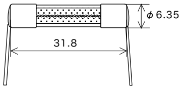
Lead wire diameter \phi 0.8 Scale: 1/1 (mm)
