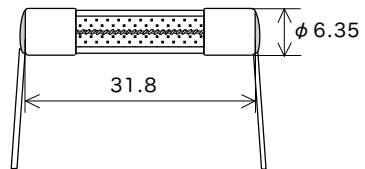
Lead wire diameter \phi 0.8 (5 A to less than 10 A) \phi 1.0 (10 A–15 A) \phi 1.2 (Over 15 A–25 A) Scale: 1/1 (mm)
