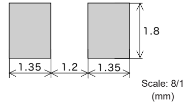
Land pattern for reflow soldering (reference dimensions)
