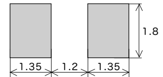
Land pattern for reflow soldering (reference dimensions)
