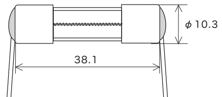
Lead wire diameter \phi 0.8 (500 mA–8 A) \phi 1.0 (Over 8 A–15 A) \phi 1.2 (Over 15 A–30 A) Scale: 1/1 (mm)
