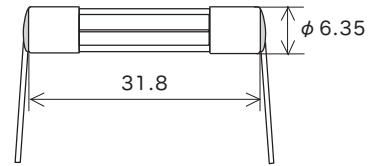
Lead wire diameter \phi 0.8 (Over 5 A–8 A) \phi 1.0 (Over 8 A–15 A) Scale: 1/1 (mm)
