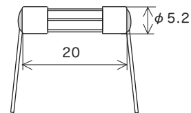
Lead wire diameter \phi 0.5 (100 mA to less than 5 A) \phi 0.8 (5 A–10 A) Scale: 1/1 (mm)
