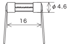
Lead wire diameter \phi 0.5 (100 mA to less than 5 A) \phi 0.8 (5 A) Scale: 1/1 (mm)
