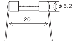
Lead wire diameter \phi 0.8
