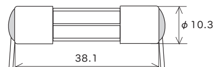
Lead wire diameter φ 0.8 (500 mA–8 A) φ 1.0 (Over 8 A–15 A) φ 1.2 (Over 15 A–30 A) Scale: 1/1 (mm)
