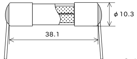
Scale: 1/1 (mm) Lead wire diameter \phi 1.2
