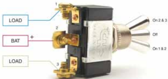
SPDT On-Off-On
